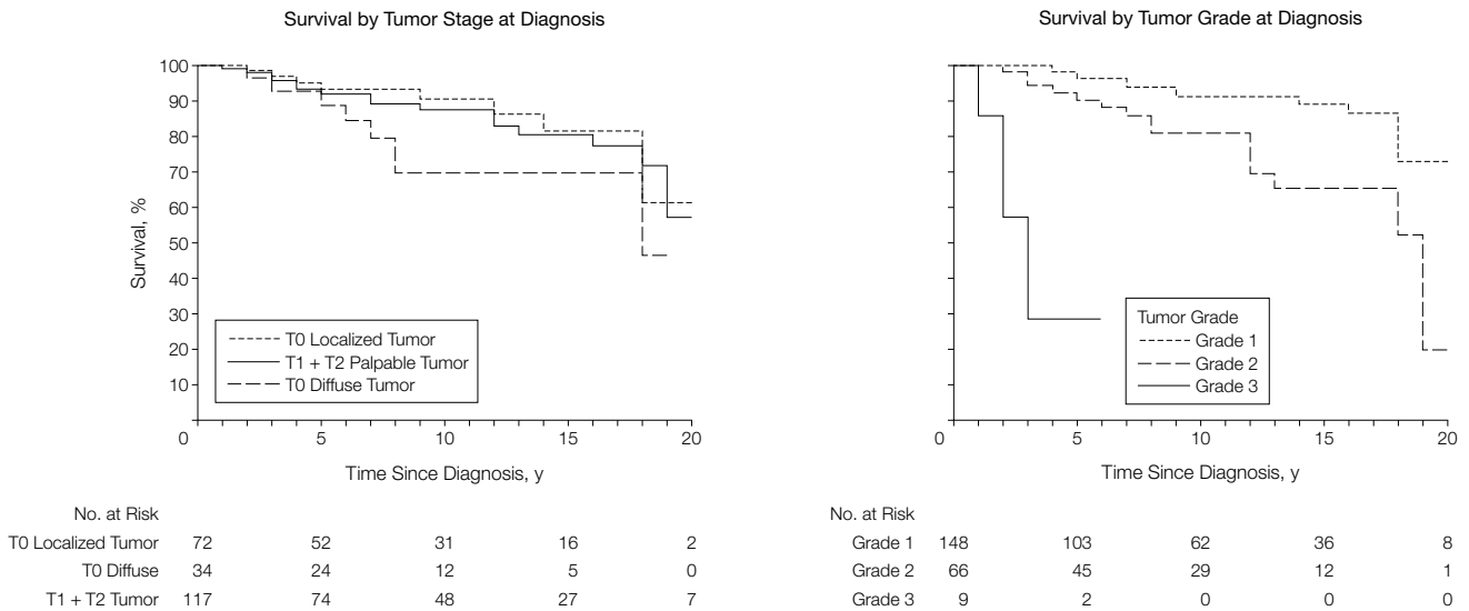
Figure 2. Cause-Specific Survival by Stage of Disease and Tumor Grade at Diagnosis
